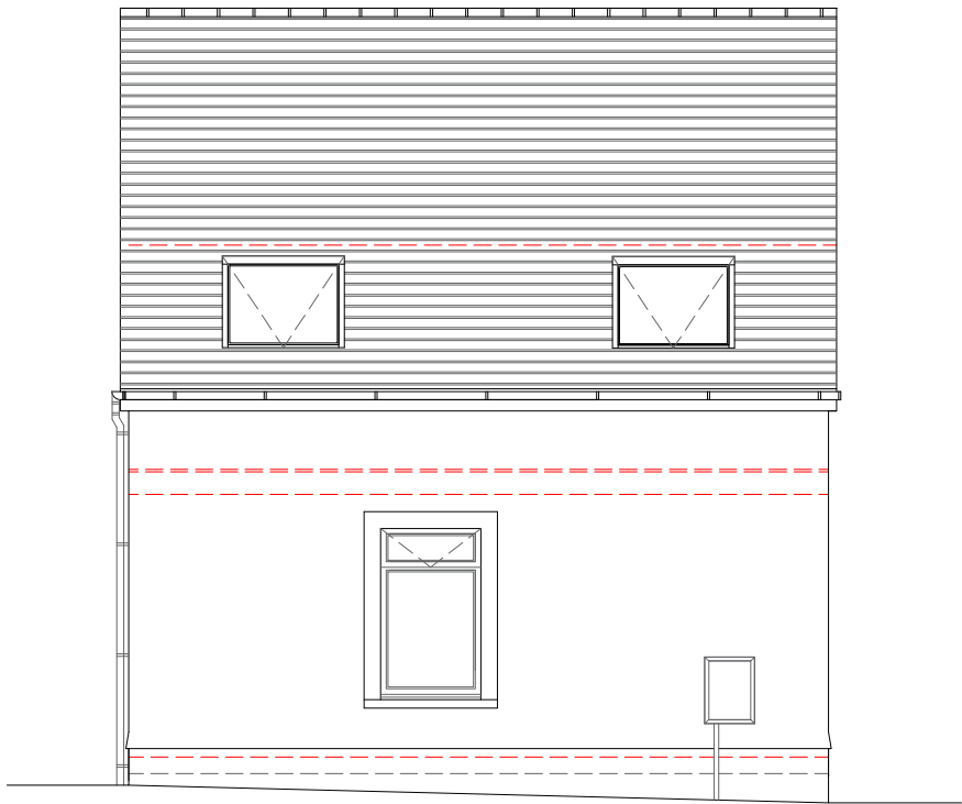
West Elevation
